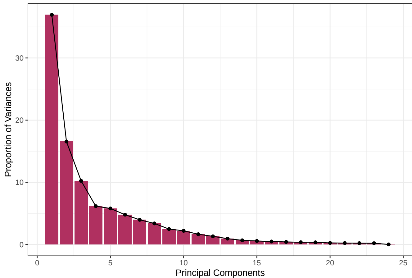
Analysis of Components Contributing to Variance
